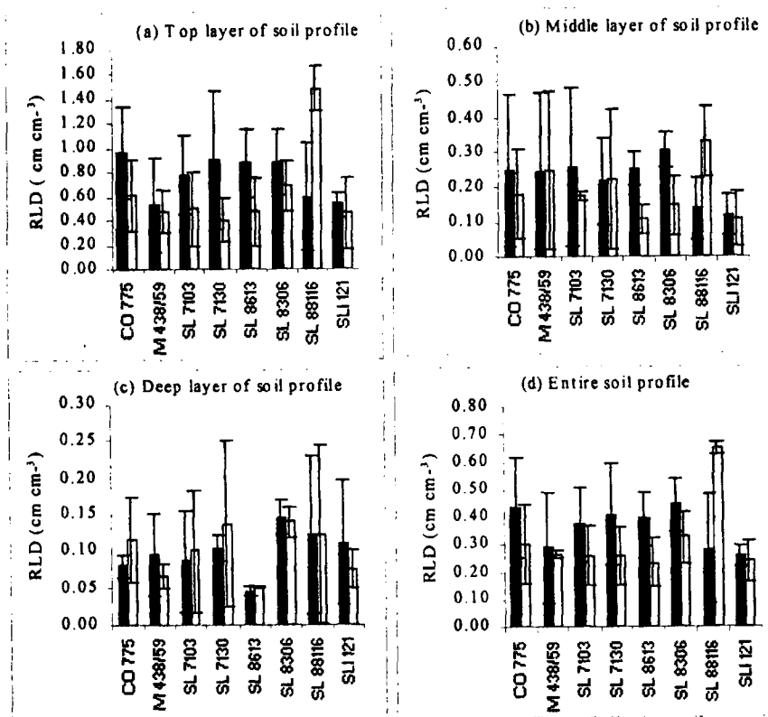
Fig. 2. Root length density (RLD) in different layers of the soil profile at 184 days after planting in different sugarcane varieties under irrigated (solid bars) and rainfed (open bars) conditions. The error bars indicate the respective standard deviations.
